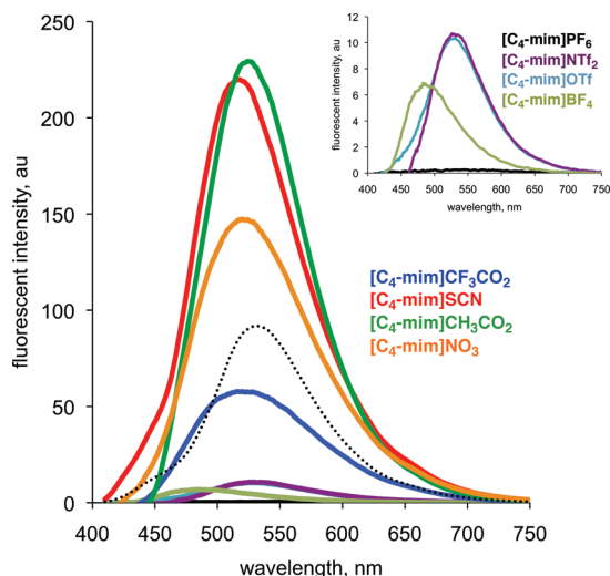
Figure 2. Emission spectra of tetracycline ( 1 , 20 \mu M) in ionic liquids (DMSO content 1% v/v); \lambda_{\text{ex}} = 400 nm. Inset shows the expanded region for [\text{C}_4\text{-mim}]\text{BF}_4 , [\text{C}_4\text{-mim}]\text{PF}_6 , [\text{C}_4\text{-mim}]\text{NTf}_2 , and [\text{C}_4\text{-mim}]\text{OTf} . The emission of 1 in DMSO (dotted line) is given for comparison purposes.
