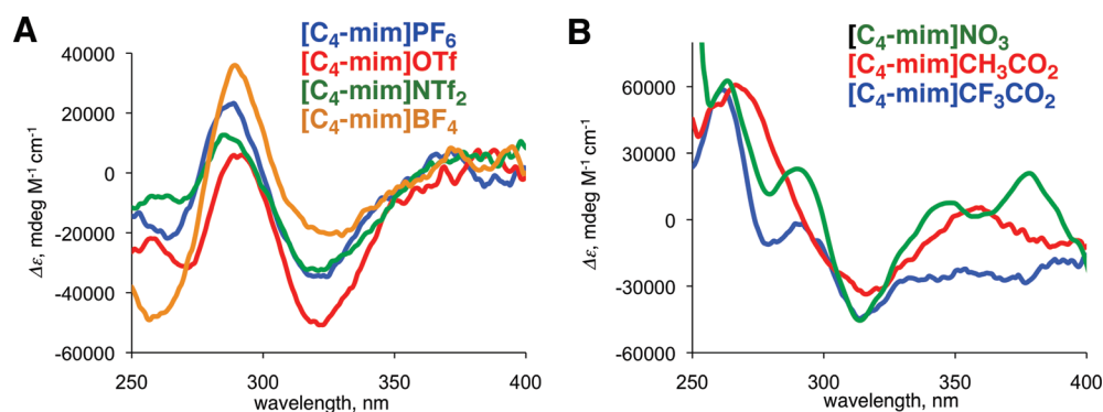
Figure 3. CD spectra of tetracycline ( 1 , 200 \mu\text{M} ) in ionic liquids (DMSO content 1% v/v).
